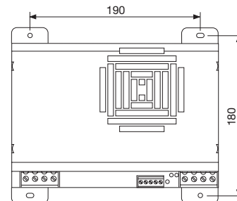
Wall mounting
